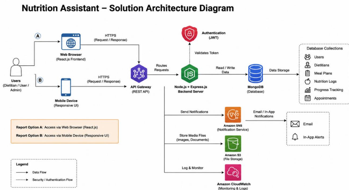
Figure 1: Solution Architecture and Data Flow of the Nutrition Assistant Application.
